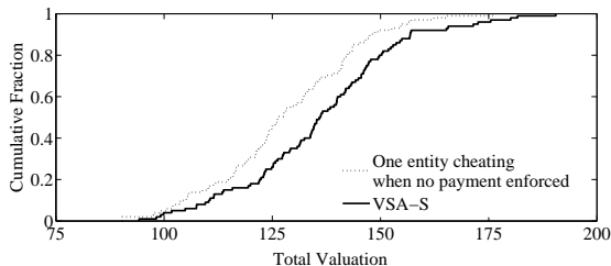
Fig. 5. Total valuation of allocated spectra in single collision domains.
