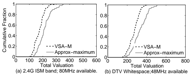
Fig. 6. Total valuation of allocated spectra in multiple collision domains.
