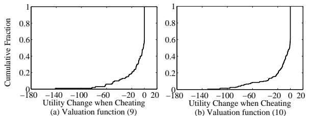
Fig. 4. Utility change for VSA-M. It shows that there is no positive utility change for cheating when VSA-M is used.
