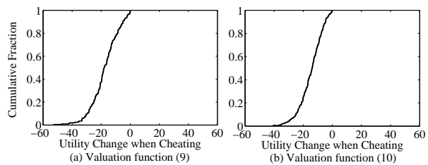
Fig. 3. Utility change for VSA-S. It shows that the utility change when cheating is never positive when VSA-S is used.
